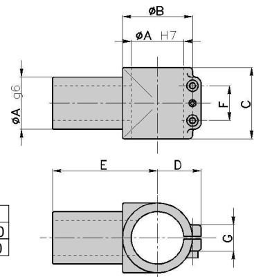
INCROCIO MASCHIO MALE CROSS BRACKET MANCHON MALE STECKHALTERUNG SOPORTE MACHO
